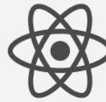
React Native
