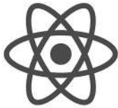
React JS
